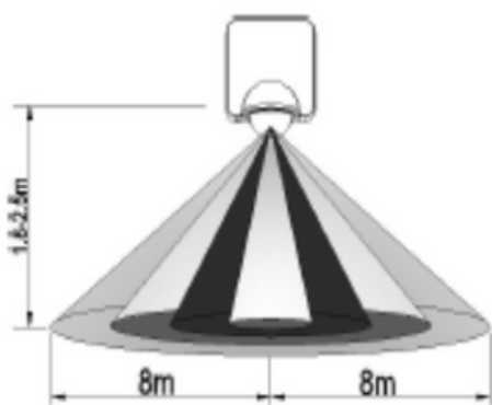
Flat mounted
